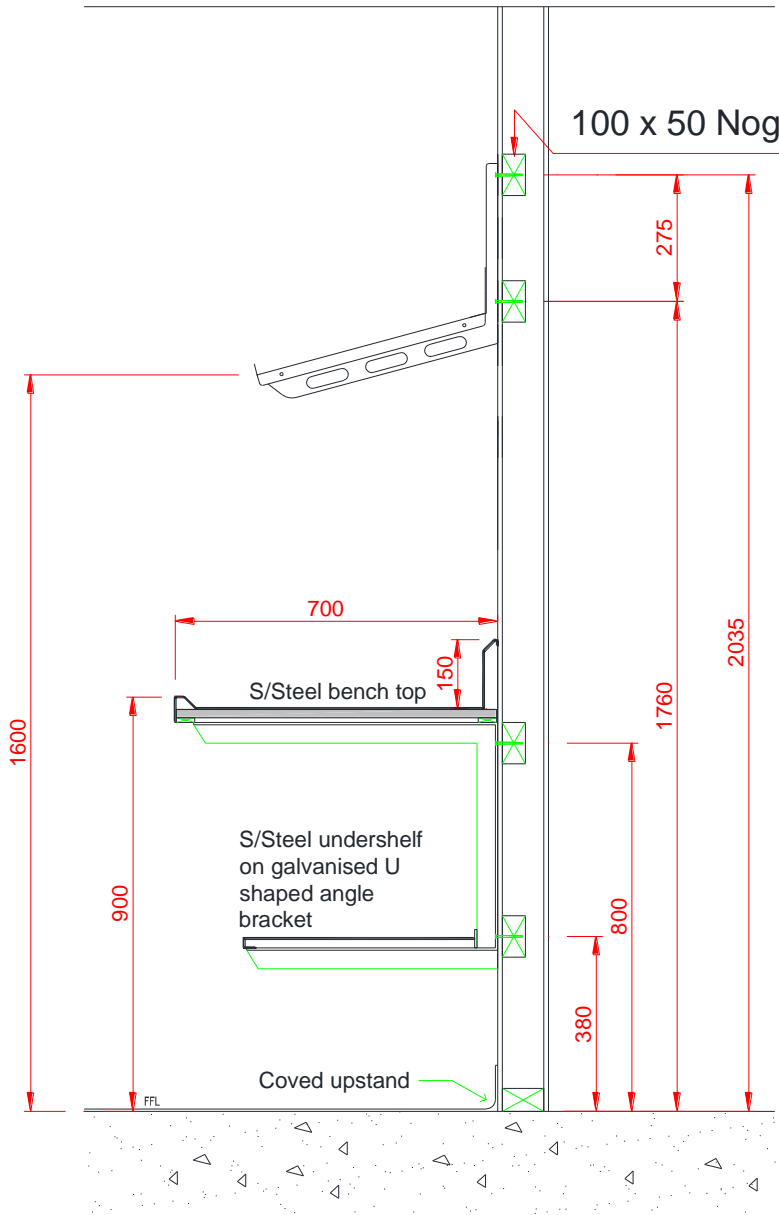
Slow moving Rack Noggin details
